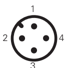
M12 connector, 4-pole
