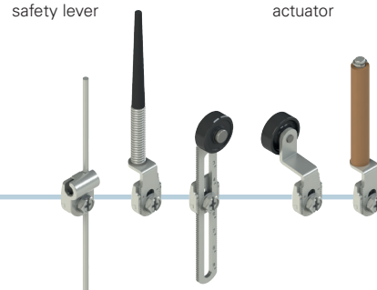
30 31 51 52 54 56 Adjustable safety lever 57 38 Without actuator
