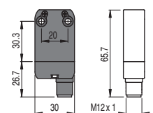
M12 connector, bottom
