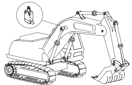
(3) - Installation in hidden position
